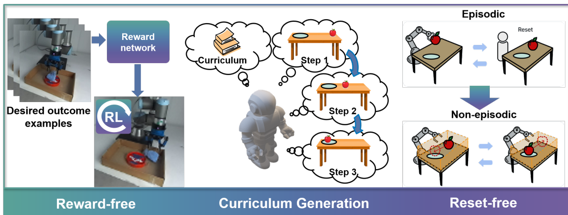
Figure 1: Minimizing external interventions for RL on embodied agents.
